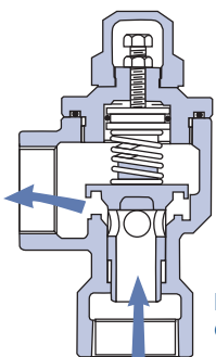
FIGURE 4. Bypass valve operation
