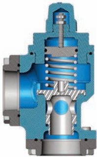
BV2 cutaway
