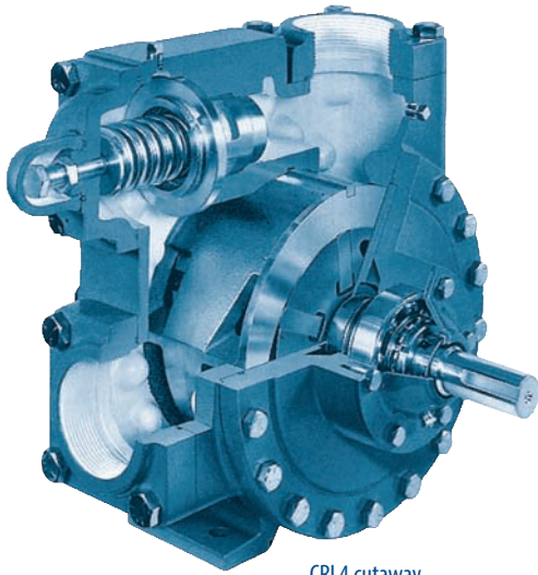
CRL4 cutaway
