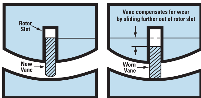
How sliding vane maintains efficiency
