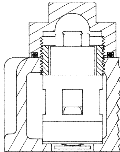
792003 (With O-Ring)
