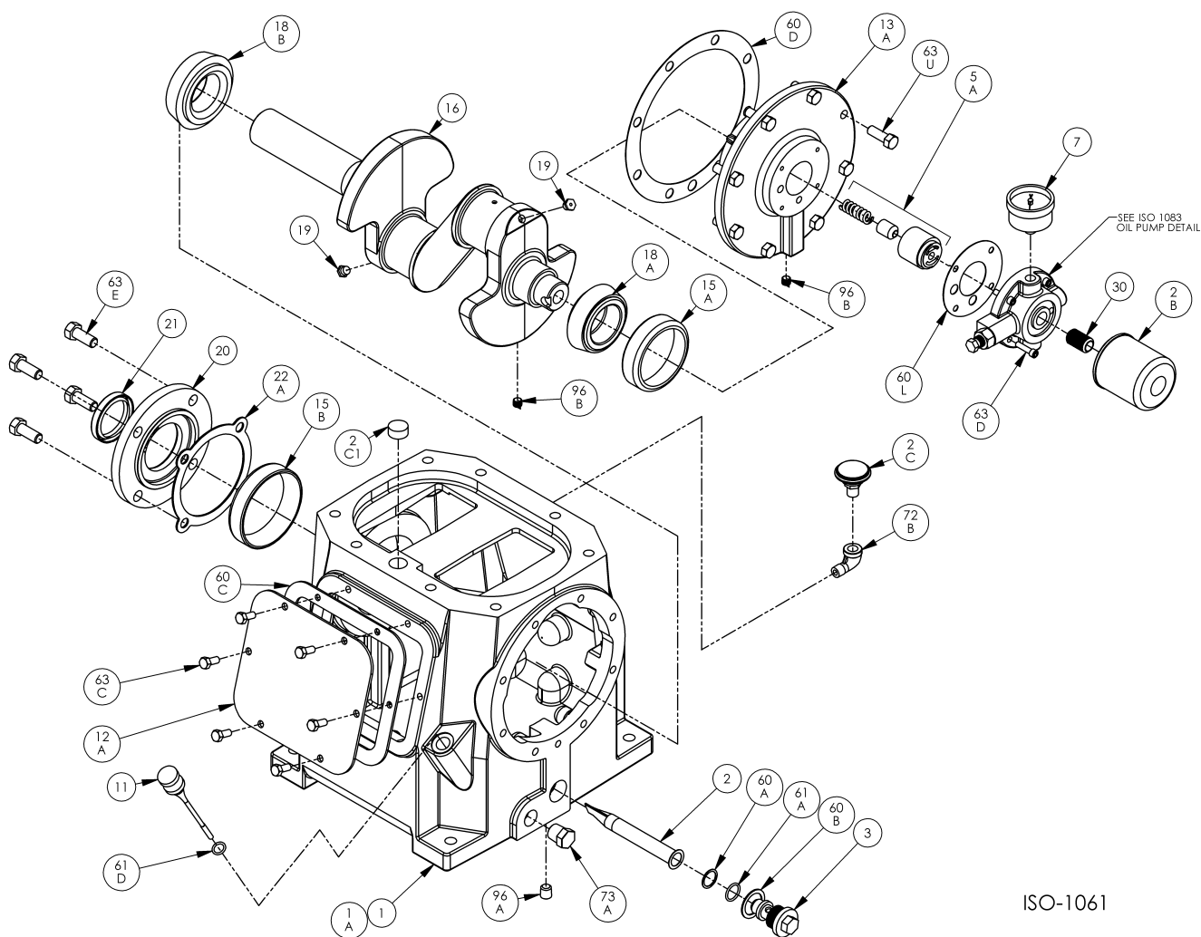
Crankcase Assembly: Models HD942A, HD942B, HDL942A, HDL942B, HD943B, HDL943B
