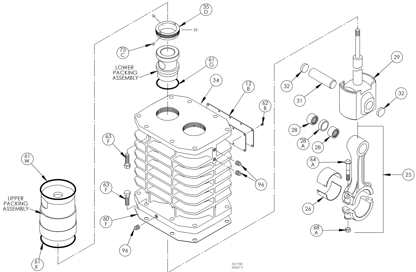
Crosshead Assembly: HD942B, HDL942B
