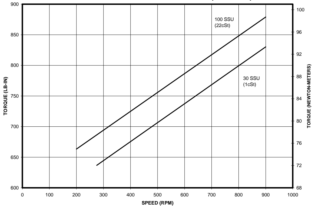
TORQUE REQUIRED AT 50 PSI (3.45 Bar)
