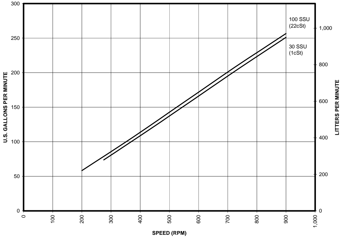
FLOW AT 50 PSI (3.45 Bar)
