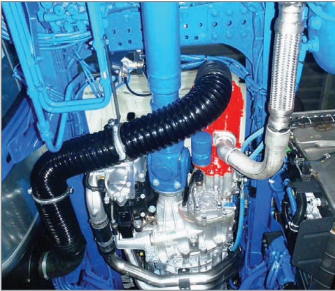
Direct mounting of the compressor assembly on the gearbox
