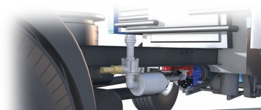
Oil cooler (supplied with flexible hoses)
