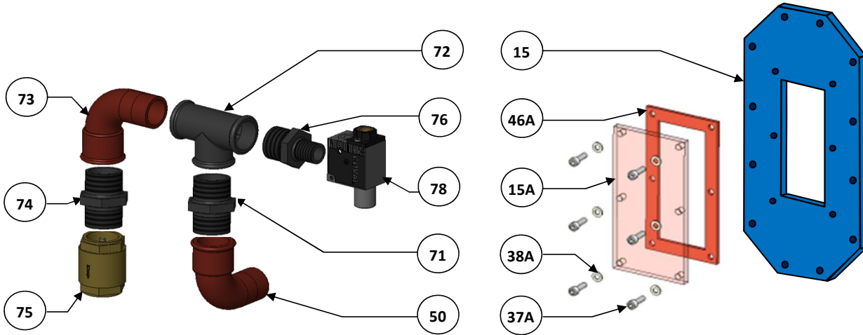
Elbow 50 : on the pump
