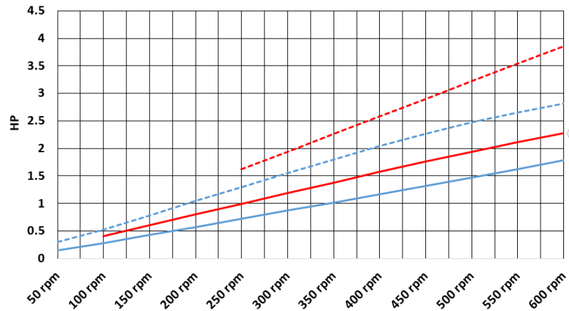
Absorbed power
