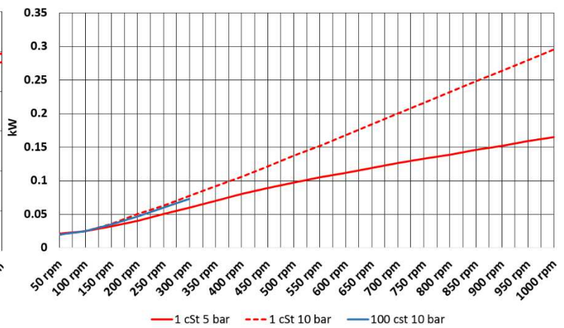
Absorbed power
