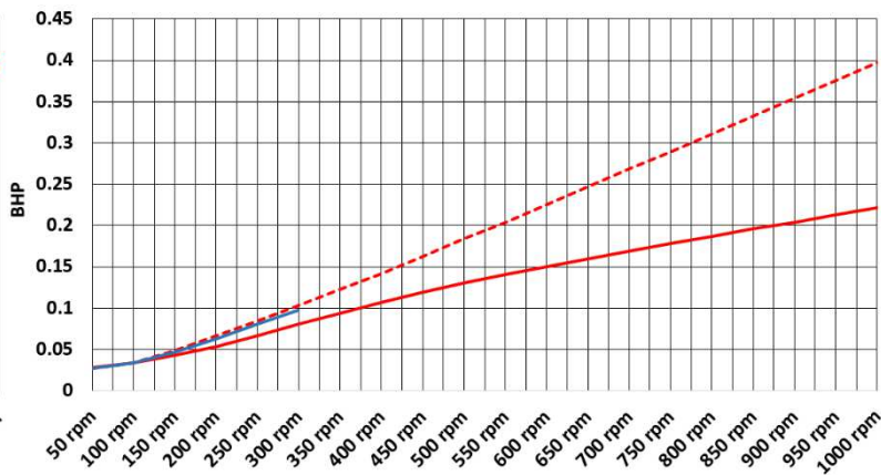
Absorbed power
