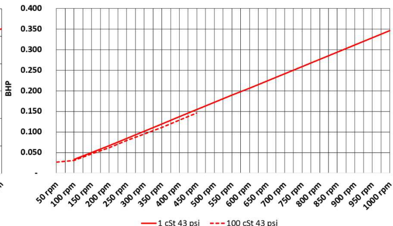
Absorbed power
