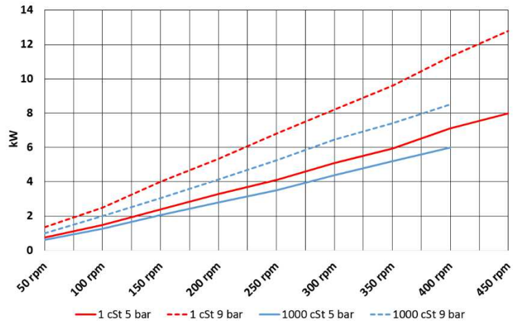
Absorbed power
