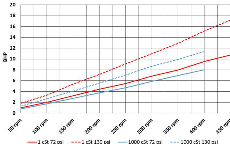
Absorbed power
