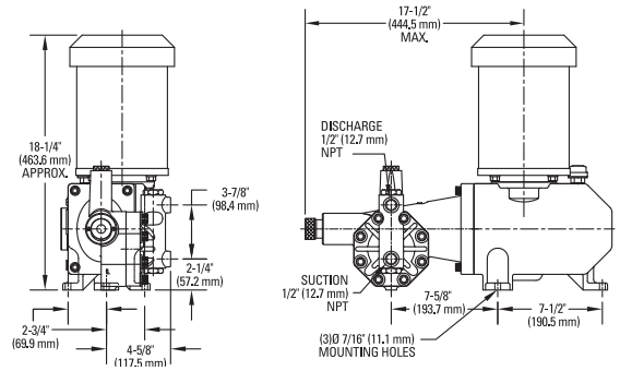
Models 6100/6150/6250 (316SS Heads)
