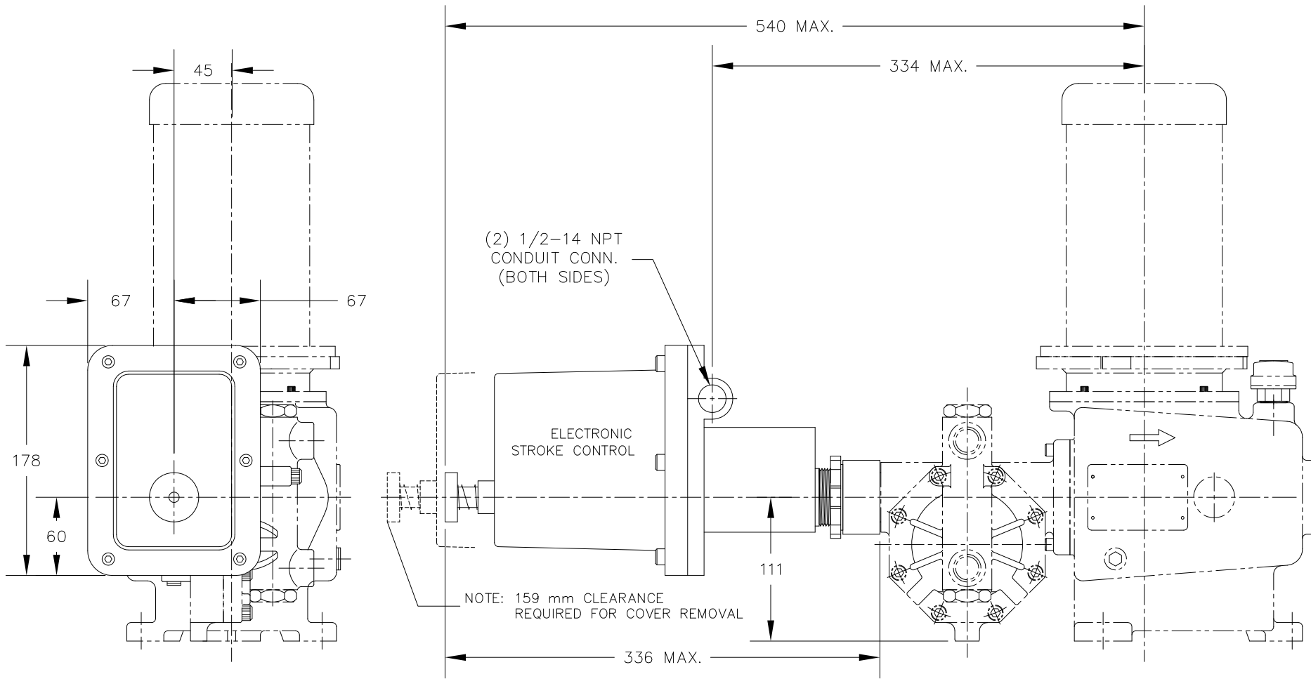
Typical Neptune dia-Pump with Electric Stroke Control
